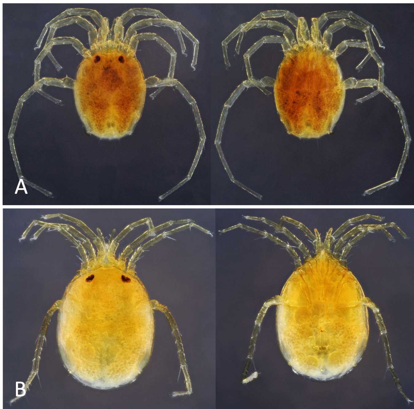
Figure 19 A – Hygrobates sp., female, dorsal and ventral view, sample site Be18-5c; B – Paraschizobates sp., female, dorsal and ventral view, sample site Be18-1b.
