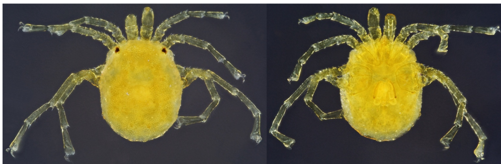
Figure 9 Sperchon sp., dorsal and ventral view, sample site Be18-10a.
