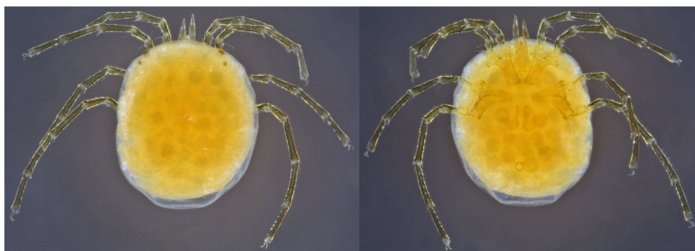
Figure 2 Hydrodroma sp., dorsal and ventral view, sample site Be18-5c.
