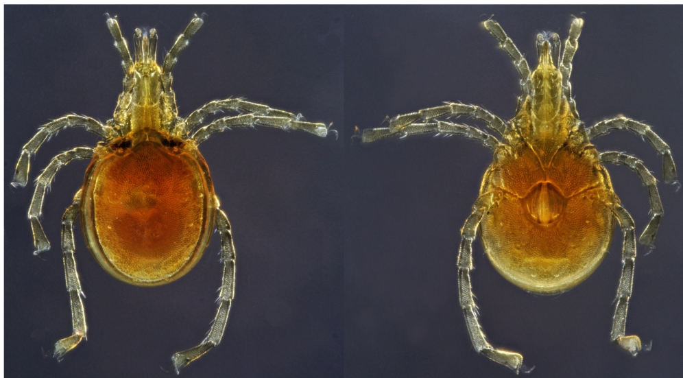
Figure 11 Neotractides sp., female, dorsal and ventral view, sample site Be18-8c.
